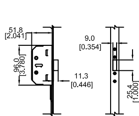
DETAIL E LATCH CASE DETAIL
