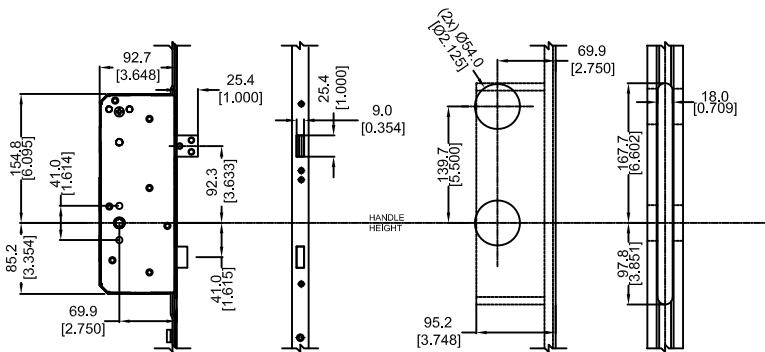
DETAIL H CENTER CASING DETAIL
