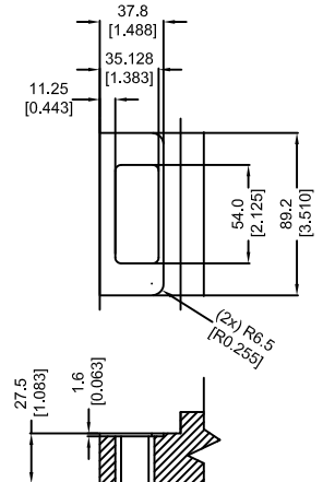
DETAIL K ADJUSTABLE STRIKE ROUTE
