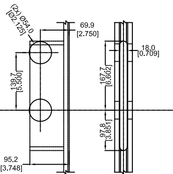
DETAIL I CENTER CASING MORTISE DETAIL
