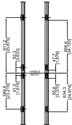
DETAIL D 6-8 LOCK STRIKE PREP
