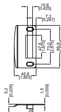
DETAIL J ADJUSTABLE STRIKE DETAIL
