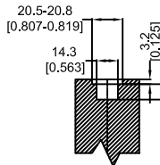
DETAIL G EUROGROOVE DETAIL
