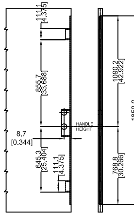
DETAIL C 6-8 LOCK DOOR PANEL PREP
