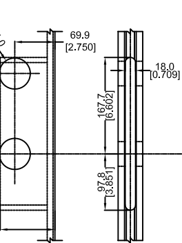
DETAIL I CENTER CASING MORTISE DETAIL
