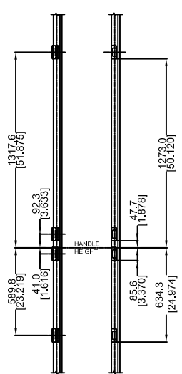
DETAIL D 8-8 LOCK STRIKE PREP
