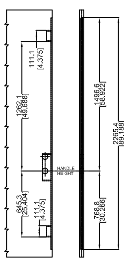
DETAIL C 8-0 LOCK DOOR PANEL PREP
