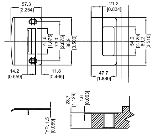
DETAIL J ADJUSTABLE STRIKE DETAIL
