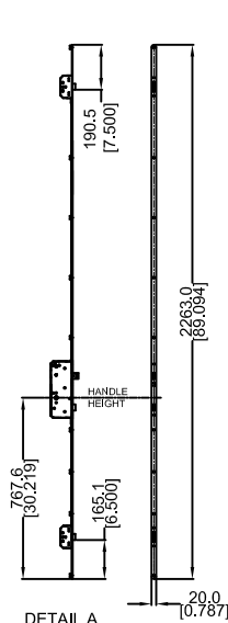
DETAIL A 8-0 TRIPLE LATCH MULTIPOINT LOCK
