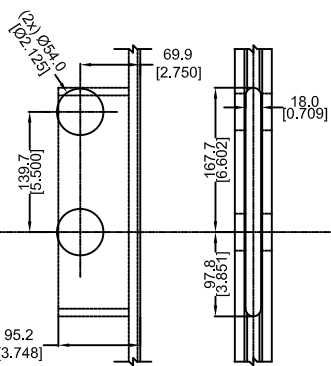
DETAIL I CENTER CASING MORTISE DETAIL
