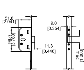
DETAIL E LATCH CASE DETAIL
