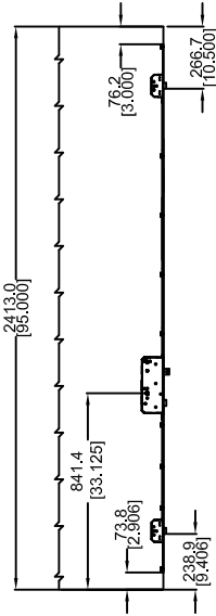
DETAIL B 8-0 LOCK SIMULATION
