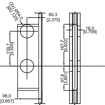
DETAIL I CENTER CASING MORTISE DETAIL
