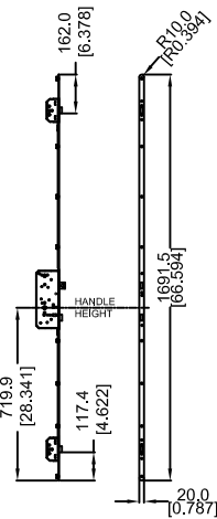
DETAIL A 6-8 TRIPLE LATCH MULTIPOINT LOCK
