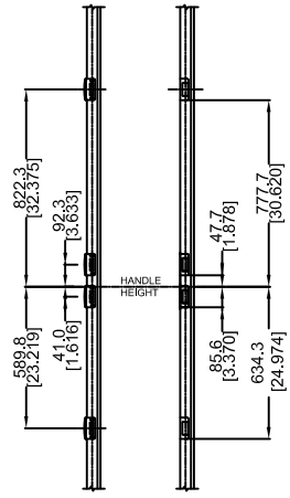
DETAIL D 6-8 LOCK STRIKE PREP
