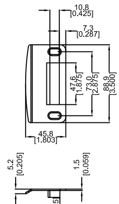
DETAIL J ADJUSTABLE STRIKE DETAIL
