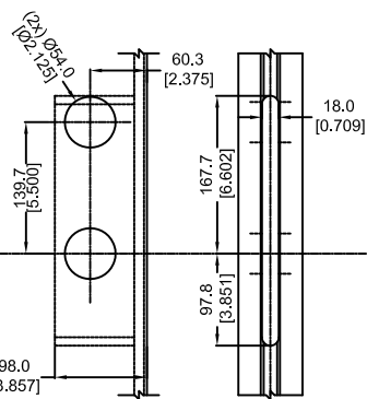
DETAIL I CENTER CASING MORTISE DETAIL
