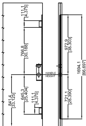
DETAIL C 6-8 LOCK DOOR PANEL PREP
