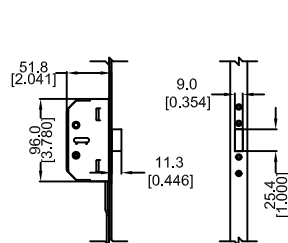
DETAIL E LATCH CASE DETAIL
