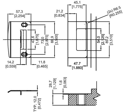
DETAIL J ADJUSTABLE STRIKE DETAIL
