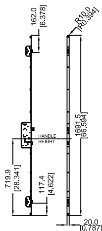
DETAIL A 6-8 TRIPLE LATCH MULTIPOINT LOCK
