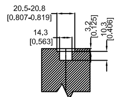
DETAIL G EUROGROOVE DETAIL
