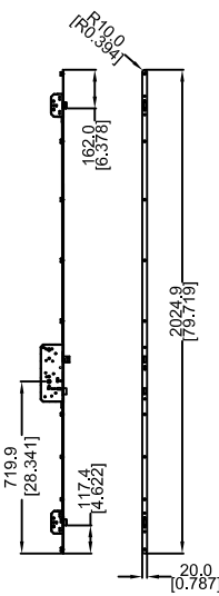
DETAIL A 8'0 TRIPLE LATCH MULTIPOINT LOCK
