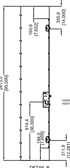
DETAIL B 8'0 LOCK SIMULATION
