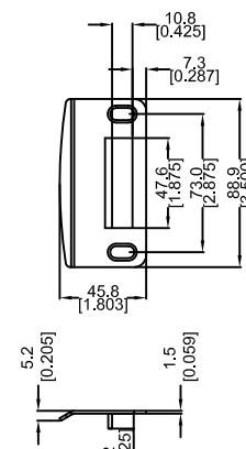
DETAIL K ADJUSTABLE STRIKE DETAIL
