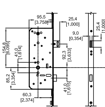
DETAIL I CENTER CASING DETAIL
