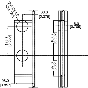
DETAIL J CENTER CASING MORTISE DETAIL
