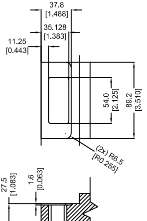
DETAIL L ADJUSTABLE STRIKE ROUTE
