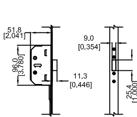
DETAIL F LATCH CASE DETAIL
