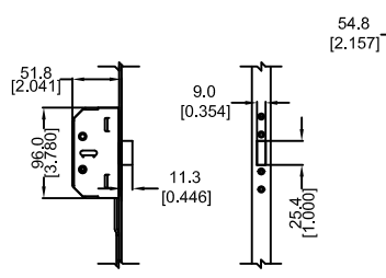
DETAIL E LATCH CASE DETAIL
