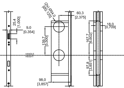
DETAIL I CENTER CASING MORTISE DETAIL
