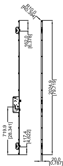
DETAIL A 8-0 TRIPLE LATCH MULTIPOINT LOCK
