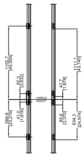
DETAIL D 8-0 LOCK STRIKE PREP
