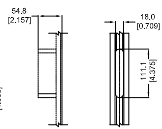
DETAIL F LATCH MORTISE DETAIL
