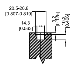
DETAIL G EUROGROOVE DETAIL
