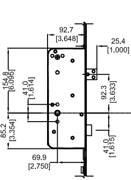
DETAIL H CENTER CASING DETAIL
