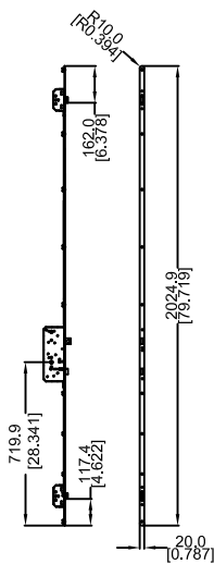
DETAIL A 8-0 TRIPLE LATCH MULTIPOINT LOCK
