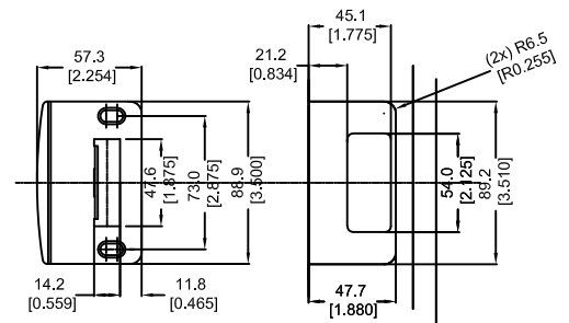
DETAIL G EURO GROOVE DETAIL
