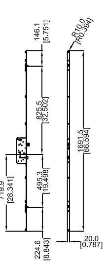
DETAIL A 6-8 TONGUE MULTIPoint LOCK
