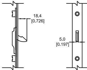
DETAIL E TONGUE DETAIL
