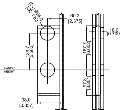
DETAIL H CENTER CASING MORTISE DETAIL
