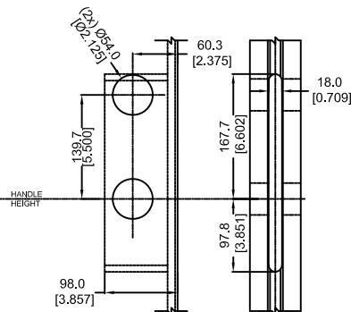
DETAIL H CENTER CASING MORTISE DETAIL
