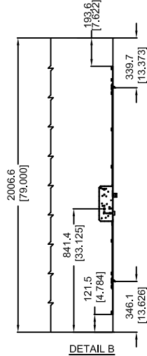
DETAIL B 6-8 LOCK SIMULATION
