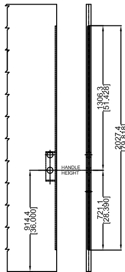
DETAIL C 8-0 LOCK DOOR PANEL PREP
