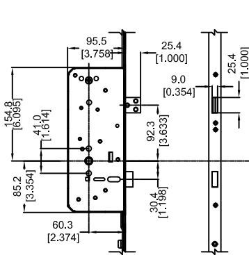
DETAIL G CENTER CASING DETAIL
