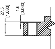
DETAIL J ADJUSTABLE STRIKE ROUTE
