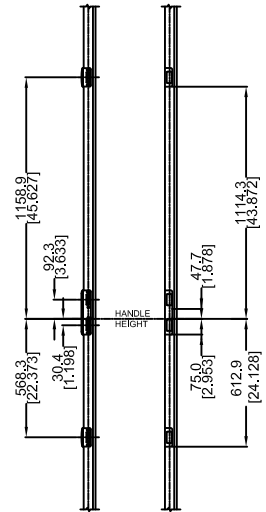
DETAIL D ADJUSTABLE STRIKE DETAIL
