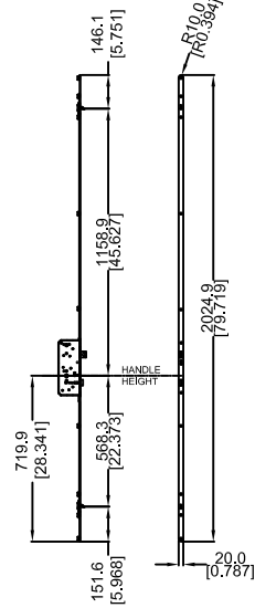
DETAIL A 8-0 TONGUE MULTIPoint LOCK
