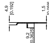
DETAIL I ADJUSTABLE STRIKE DETAIL
