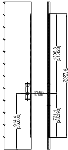
DETAIL C 8-0 LOCK DOOR PANEL PREP
