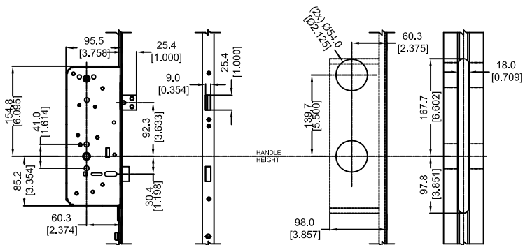
DETAIL G CENTER CASING DETAIL
