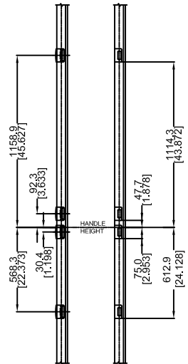
DETAIL D ADJUSTABLE STRIKE DETAIL
