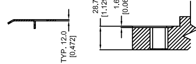
DETAIL J ADJUSTABLE STRIKE DETAIL
