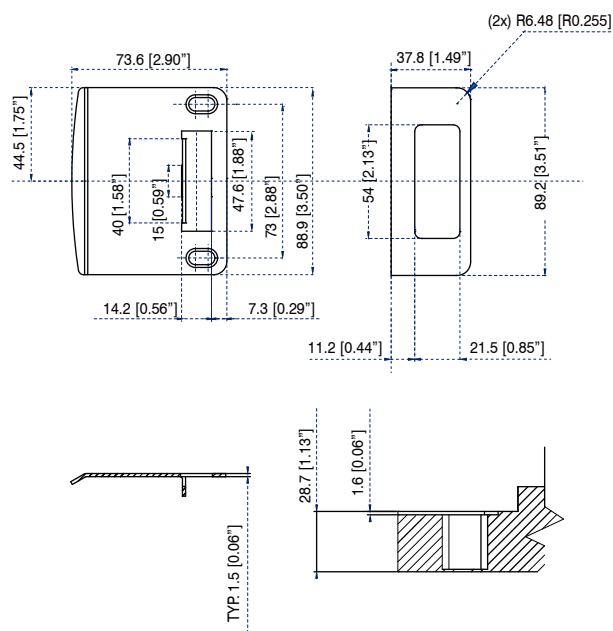
Dimensions and Routing Detail
