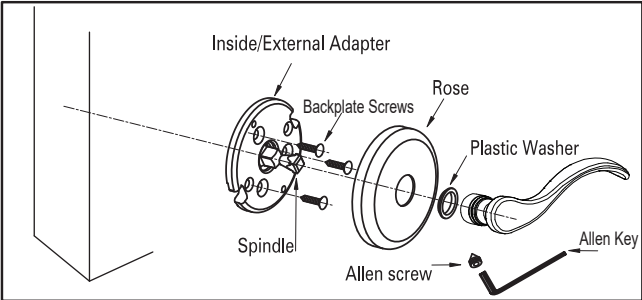
Exploded View Dummy Lockset
