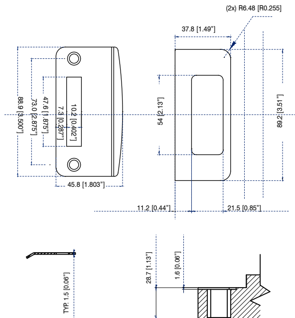
Dimensions and Routing Detail
